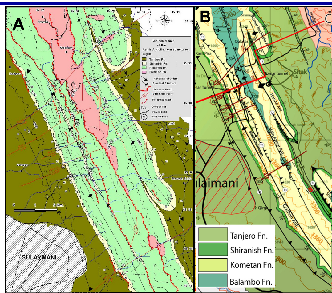
Fig.(5) Geological map of the studied area, A) Omer (2011) B) Al-Hakari (2011)
