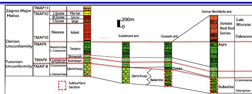
Fig.(2) Correlation of the Cretaceous formations (Al-Hakari, 2011) which shows that Gulneri Formation is not deposited in the studied area and Dokan is deposits on Goizga anticline only
