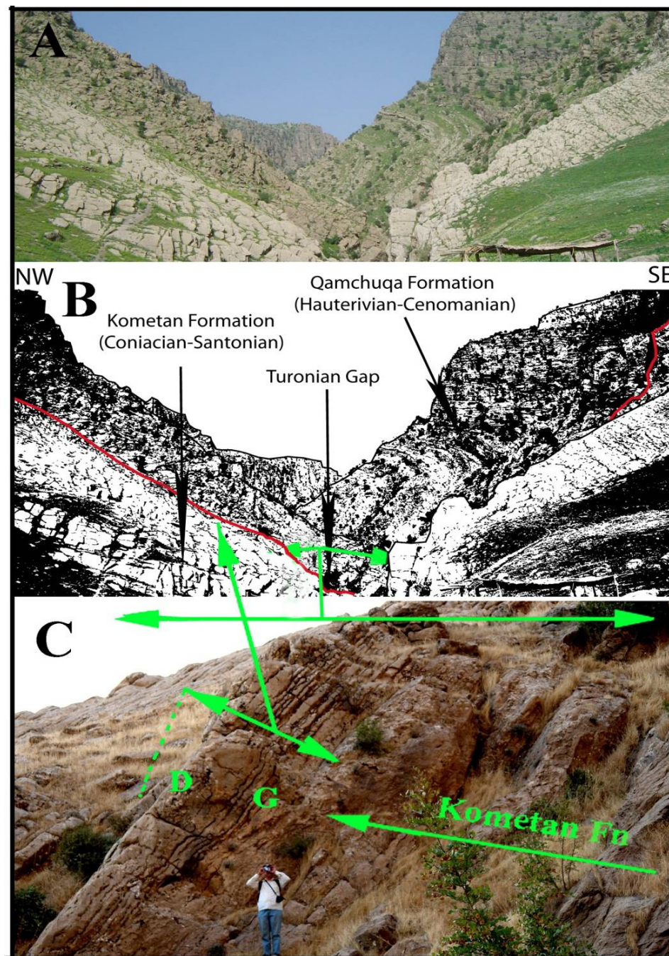
Fig. (20) A and B) photo of Lawa et al. (2013) for indication that Dokan and Gulneri formation are not present (Unconformity for 4.7 m.y) in the Tabeen Gorge 4km to the southeast of Surdash village. C) Photo of the same gorge of the present study which shows clearly that equivalents of both formations (EODF and EOGF) are existing and only the facies are changed which means that there are not unconformity. The EODG appear as highly deformed and thin bedded limestone under Kometan Formation.
