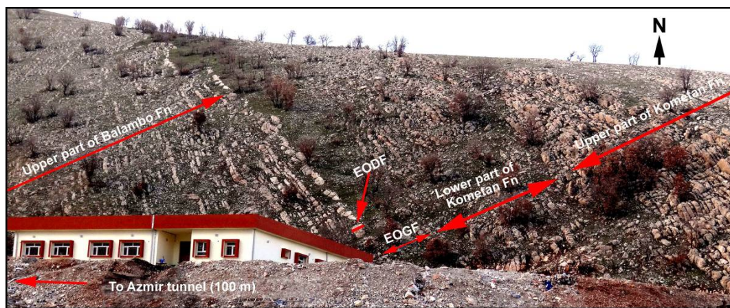
Fig.(7) Kometan and Balambo Formations with EOGF and EODF in between along the northeastern limb of Azmir-Goizha anticline near out let of Azmir tunnel.
