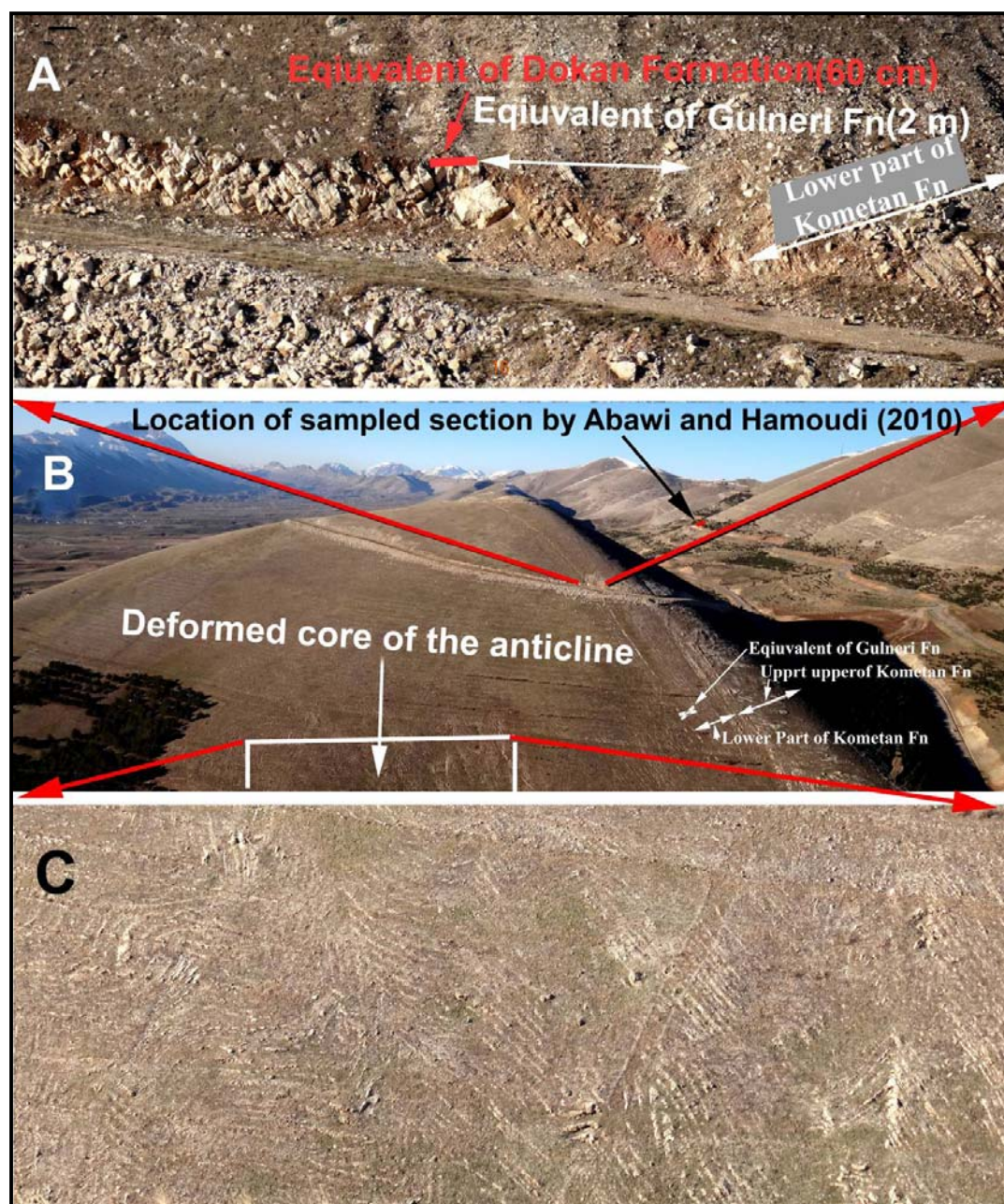
Fig.(8) A, B) EOGF and EODF along the Salta Re Hill (Naugirdan hills). C) Deformed core (Balambo Formation) of the above mentioned hill.
