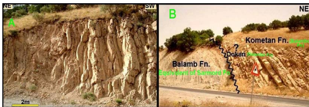
Fig. (10) Due to complexity of the studied area the confusing is clear in the identification of the Formation. A) Vertical of beds Balambo Formation which is identified by Al-Hakari (2011, p.83) as Kometan Formation on the eastern side of the paved between Sulaimani city and Chwarta town. B) A photo (by the latter author) shows Turonian unconformity, Balambo and Kometan Formations. In the present study they are changed to conformity, Sarmord and Balambo Formations respectively as shown by green fonts.
