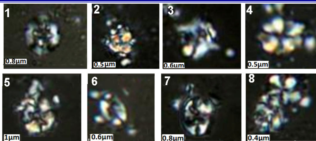
Fig. (11) Species of nannofossils in the Equivalent of Gulneri Formation (EOGF) which gave the age of Turonian. 1- Retecapsa angustiformata (S. 2MBK), 2- Radiolithus planus (S. 2MBK), 3- Prediscosphaera columnata (S. 1 MBK), 4- Eprolithus moratus (S.5 MBK), 5- Eiffellithus eximius (S.4 MBK), 6- Eiffellithus gorkae (S.4 MBK), 7- Eiffellithus turriseiffelli (S.4 MKB), 8- Eprolithus Moratus (S. 4 MBK)
