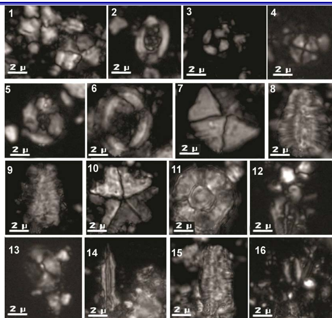
Fig. (19) Extracted nannofossils in the five samples of Qaywan valley where both age and lithology prove occurrence of Sarmord Formation. The ages that are indicated by these fossils are upper Berriasian, Lower Valanginian, Lower Hauterivian and Upper Barremian. 1- Carinolithus magarensis (s1), 2- Crepidolithus granulates (s1); 3- Diazomatolithus lehmanii (s1), 4- Discorhabdus ignotus (s1), 5- Helenea chiastia (s1); 6- Manivitella pemmatoidea (s1); 7- Micrantholithus hoschulzii (s1); 8- Nannoconus steinmannii minor (s1); 9- Nannoconus kamptneri (s2); 10- Micrantholithus obtusus (s3), 11- Nannoconus sp. (s3); 12- Staurolithites sp. (s3); 13- Haquis ellipticus (s3); 14- Lithraphidites carniolensis (s3); 15- Faviconus multicolumnatus (s3); 16. Rhagodiscus pseudoangustus (s14).
