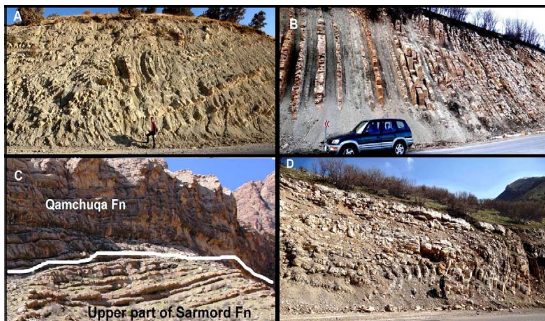
Fig.(17) A and B) Outcrops of Sarmord Formation in the northeast of Azmir-Goizha anticline (locally called Qaywan anticline) which assumed to be Balambo Formation by all previous studies and in the present study nanofossils prove Early Barremian age of this location. C) Upper part of the formation at its type area which can be compared with those of the studied area. D) Balambo Formation, Azmar Mountain (Al-Qayim et al , 2012, fig.11c and 25a) which changed to Sarmord Formation in the present study. The section consists of alternation of marl and marly limestone (Note: The mountain is Qaywan not Azmar (Azmir)).
